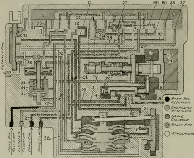
FIG. 6. EMERGENCY POSITION-TRIPLE VALVE IN QUICK RELEASE
